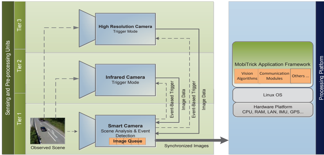
Fig. 1: High-level architecture of the traffic surveillance system
