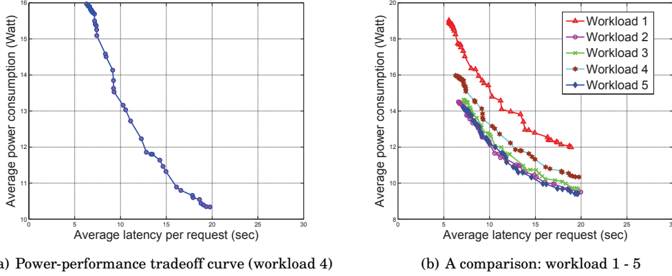
Fig. 7: Pareto-optimal tradeoff curves of different workloads
