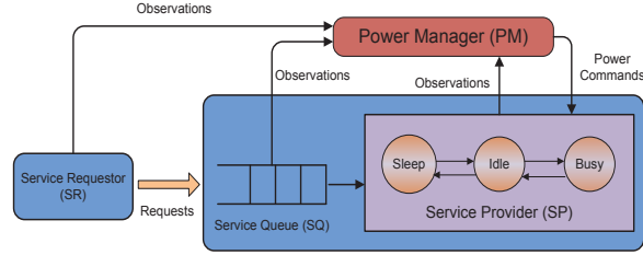
Fig. 2: Generic DPM model
