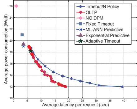
Fig. 9: Comparison of the OLTP with different DPM policies
