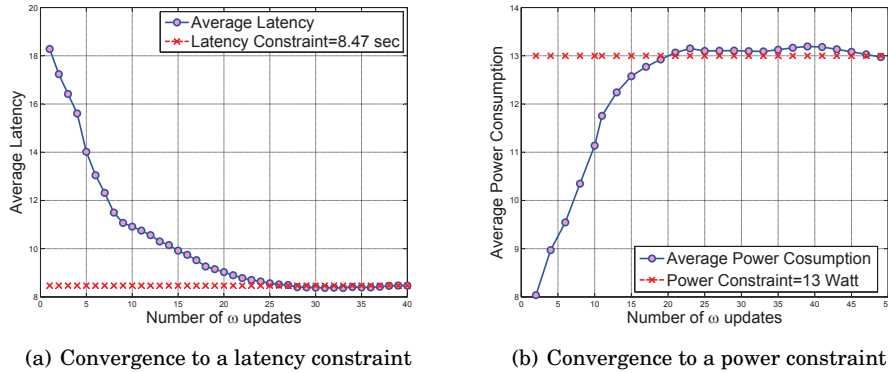
Fig. 11: Power-performance weight adaptation for latency and power constraints
