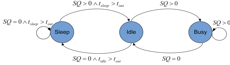
Fig. 4: System state-transition diagram
