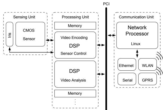
Fig. 1. The hardware architecture of our smart camera.
