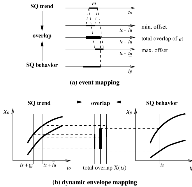
Fig. 13. The effect of time uncertainty t_u in trend/behavior mapping. In the presence of time uncertainty the SQ trend can be shifted from the SQ behavior by any time offset within the time uncertainty ( t_p = t_o - t_u ). Time uncertainty increases the time overlap between the SQ trend and the SQ behavior of events (a) and the magnitude overlap of dynamic envelopes (b). These broader bounds weaken the refinement process.
