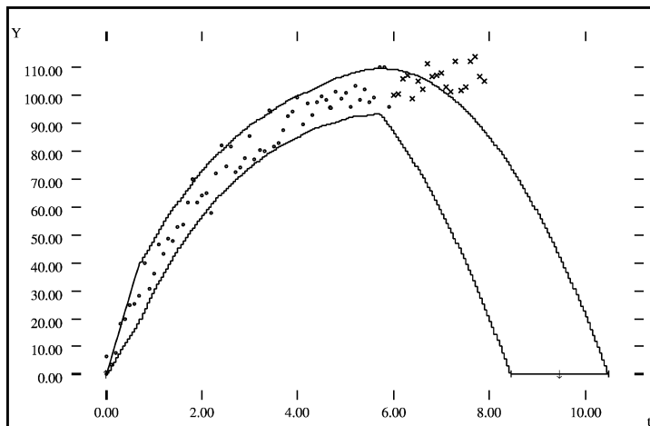
Fig. 18. Structural mismatch between data and model. At up to 60 points (dots), SQUID finds a portion of the initial model space that is consistent with the measurements. After 80 points (crosses), SQUID is able to refute the model because no extrema was detected in the data before the end of the simulated maximum, i.e., event mapping resulted in an empty overlap.
