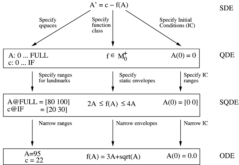
Fig. 1. Multi-level model of an imprecisely-known system based on the QSIM representation. At each level, the representation entails a space of ODEs. At the top is the purely structural SDE. The QDE adds qualitative information to the SDE, and the SQDE adds imprecise numerical information to the QDE. As we move downward we specify more information, thus reducing the size of the model space.
