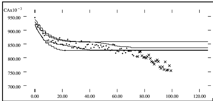
Fig. 19. Refuting a drifting fault in a CSTR. The inner dynamic envelope is generated from data up to t = 70 . The outer envelope is generated from the original SQDE. Note that the model is clearly in error from t = 70 onward.
