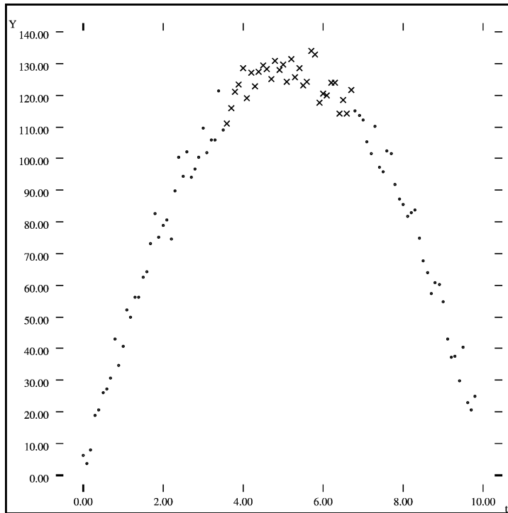
Fig. 7. Binning a simulated measurement stream ( y'' = -9.8 , y(0) = 0 , y'(0) = 50 with added Gaussian noise with variance \sigma^2 = 5 ). Binning finds three regions for this data—one maximum ( \times 's) surrounded by two monotonic regions.
