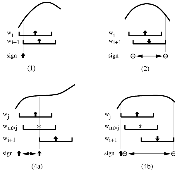
Fig. 5. Determining signs (of data-points) from kernel values (of windows). Numbers in parentheses refer to the corresponding cases in the text.
