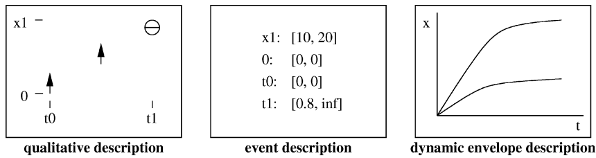
Fig. 2. The SQ behavior description. SQSIM derives behavioral components at the qualitative, event and dynamic envelope level.
