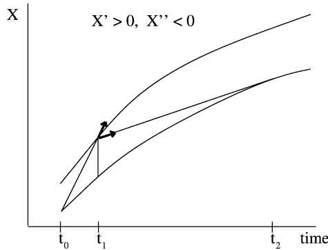
Fig. 9. Computing bounds on the derivative of a state variable from its dynamic envelopes. The signs of the first and second derivatives of x provide information to determine bounds on x' from the dynamic envelope of x .
