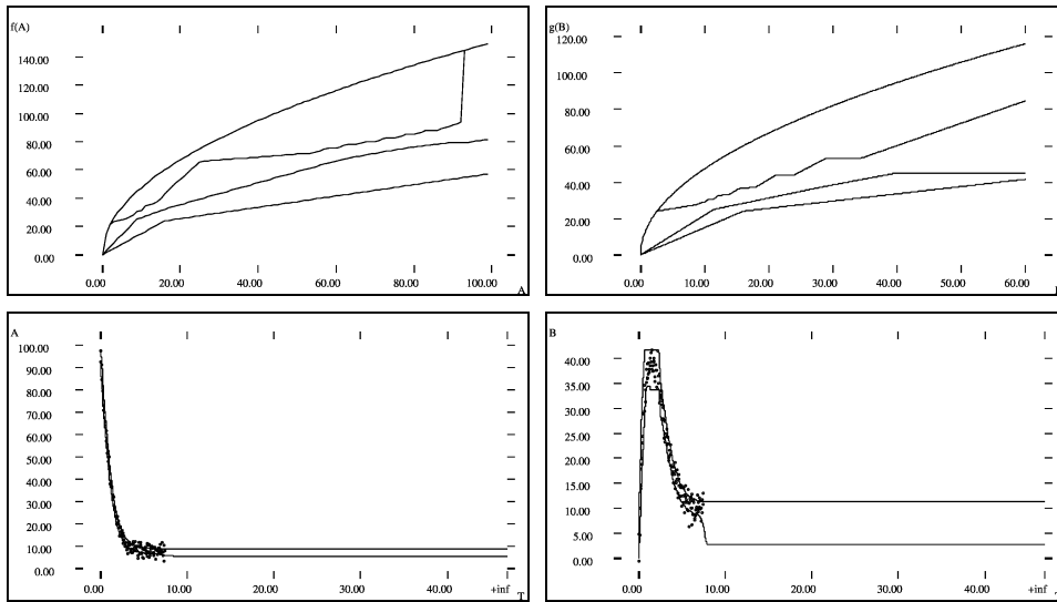
Fig. 17. Refinement of the static envelopes f and g (top) and the predicted dynamic envelopes A and B (bottom) in the two-tank cascade when A , B , f(A) , and g(B) are measured. The outer envelopes in the upper graphs are the initial ones provided by the SQDE. The measurements for A and B are plotted in the lower graphs.
