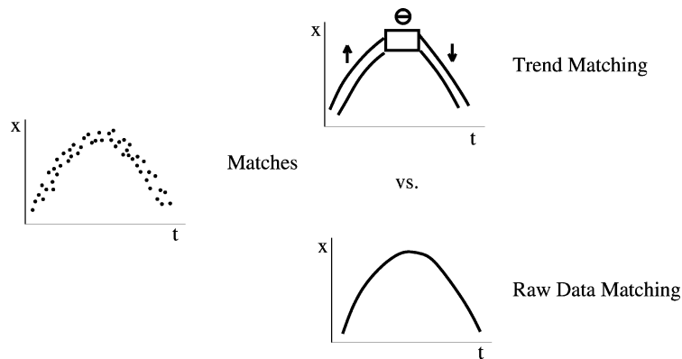
Fig. 4. Trend matching uses abstract properties of the observation (monotonicity, location of events, and dynamic envelopes) to compare data to models (top). Traditional methods use specific function matches for comparison (bottom).
