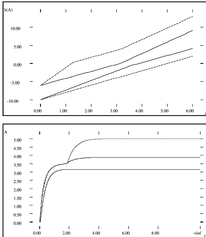
Fig. 16. The effect of collapsing uncertainty sources. Using the single uncertainty source h(A) rather than f(A) - C leads to improvements in both the bound on h(A) (upper graph) as well as the predicted trajectory whose upper equilibrium bound shrinks from \sim 5.0 to \sim 3.9 (lower graph). Dashed lines in the upper graph correspond to multiple-source uncertainty f(A) - C , the solid lines correspond to the refined static envelope of the collapsed multiple-source uncertainty h(A) .
