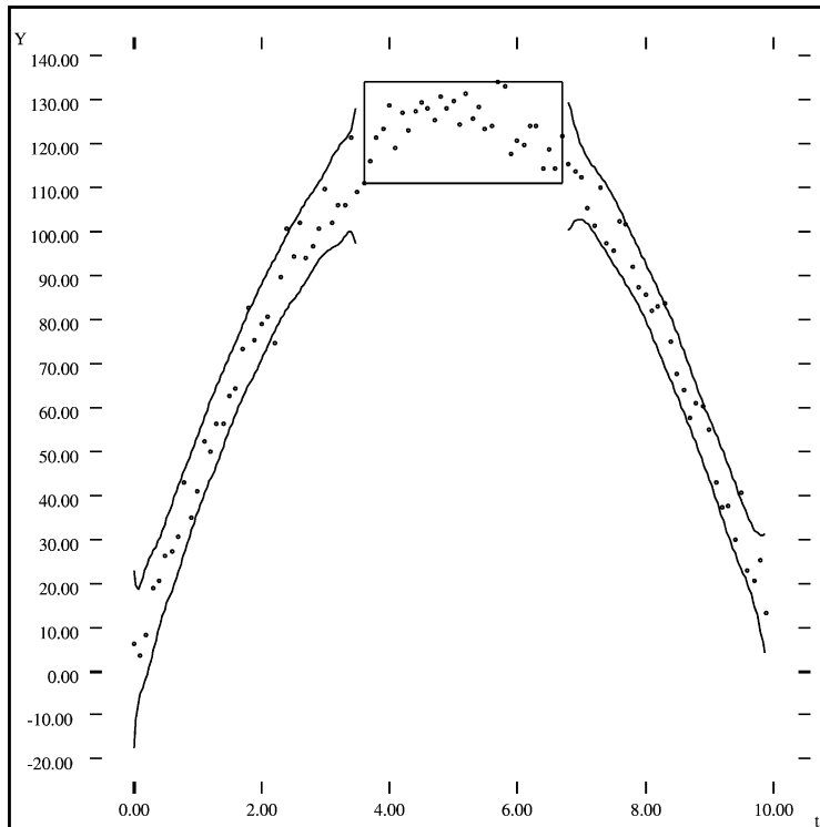
Fig. 8. Fitting bins. Each \ominus bin is bounded by the smallest box that includes all points in the bin. Each monotonic bin is enclosed by bounding envelopes generated by the neural network-based function estimator MSQUID.
