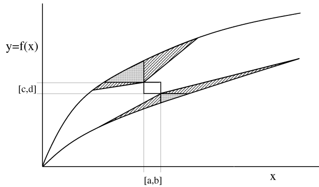
Fig. 11. Refining a static envelope. Monotonicity requires that an increase in x leads to an increase in y . Thus, if the region in the box contains a point on f(x) , the dark-shaded regions cannot contain parts of the function. Curvature information about f(x) allows a further refinement, i.e., the elimination of the light-shaded regions for a concave down function.
