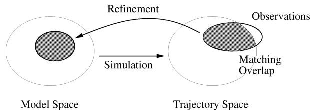
Fig. 3. Refinement matches observations to the trajectory space of a corresponding model space. It then infers a smaller model space that is consistent with the smaller trajectory space. In traditional identification, this process is simplified because only one trajectory is compared at a time, so the simulation and refinement operators are easy to implement.
