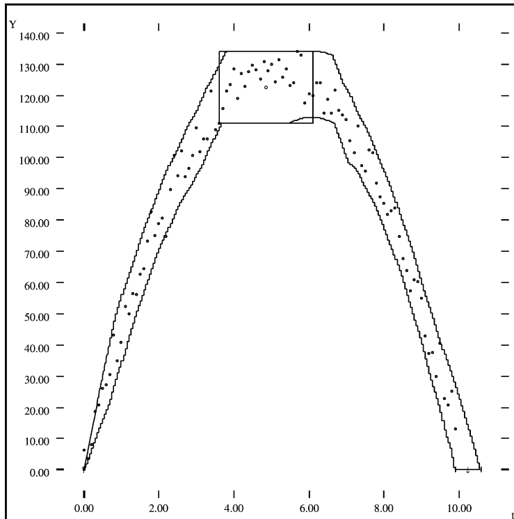
Fig. 10. The predicted trajectory of the gravity model after refinement. The bound on initial velocity has been reduced from [20, 60] to [36.3, 60] . Note that the bound for y near t = 0 is better than that of the trend dynamic envelope (Fig. 8) since the model prediction provides greater constraining power than do the measurements at that time.
