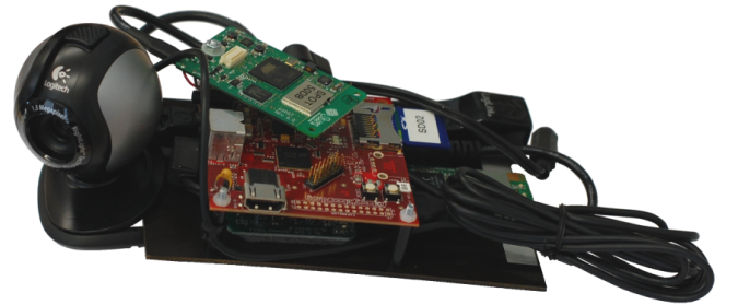
Figure 2: A Pervasive Smart Camera prototype with an embedded processing board, a webcam, an 802.11 radio and a SunSPOT for 802.15.4 connectivity.
